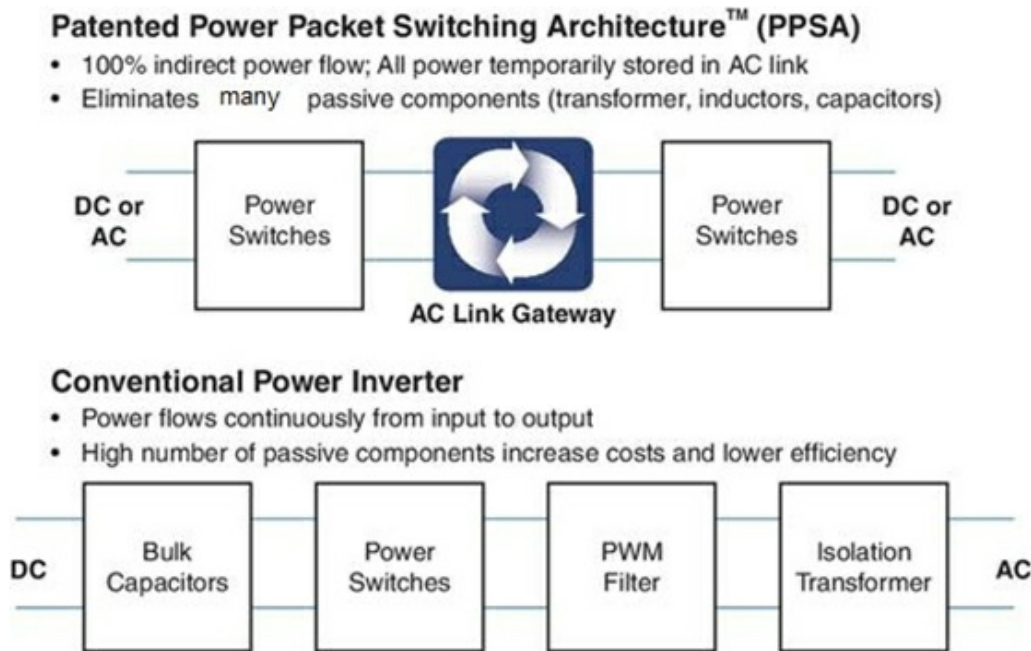
Figure 1: Schematic of PPSA Process
